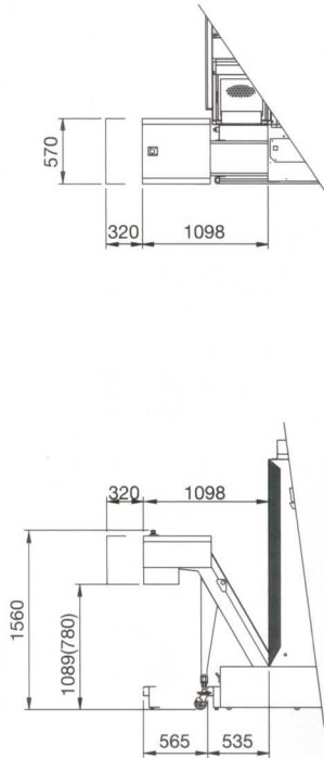
chip conveyor
